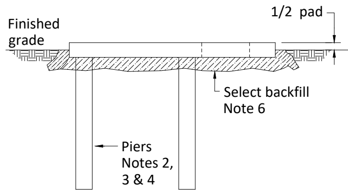
Side View for Level Terrain
