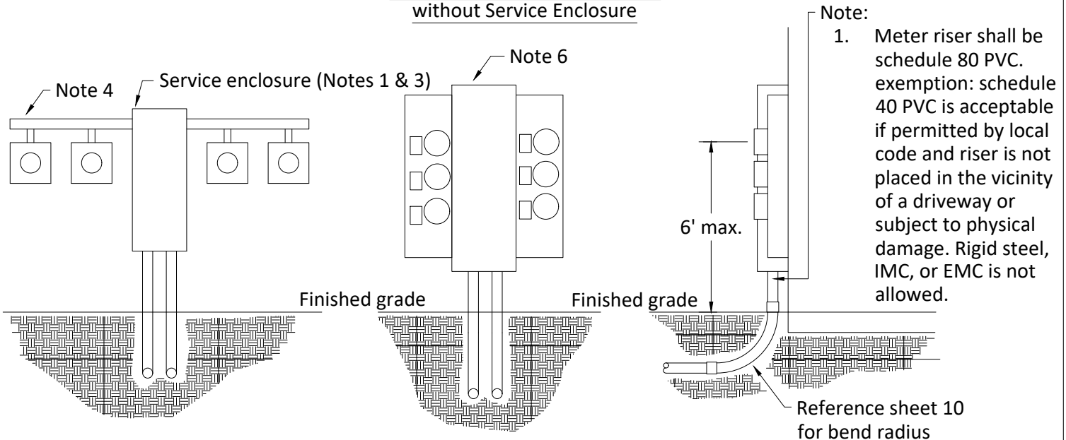
Typical Gang Meter with Service Enclosure
