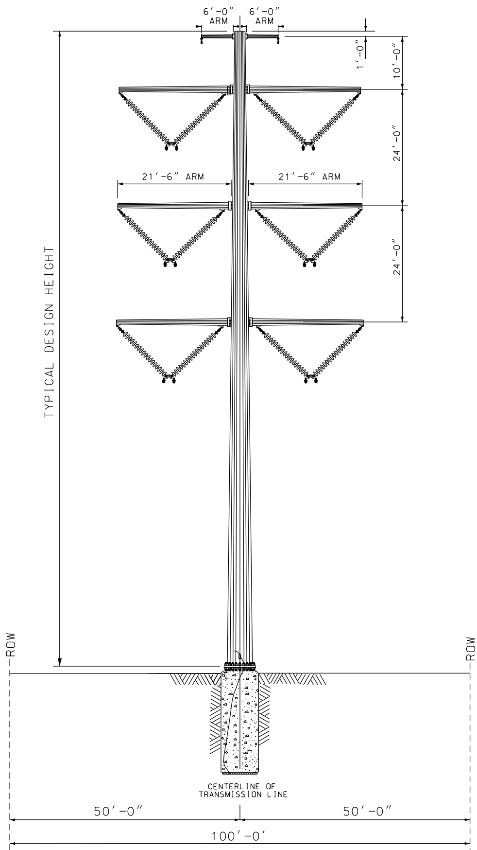
TYPICAL 345 KV TANGENT DOUBLE CIRCUIT MONOPOLE
