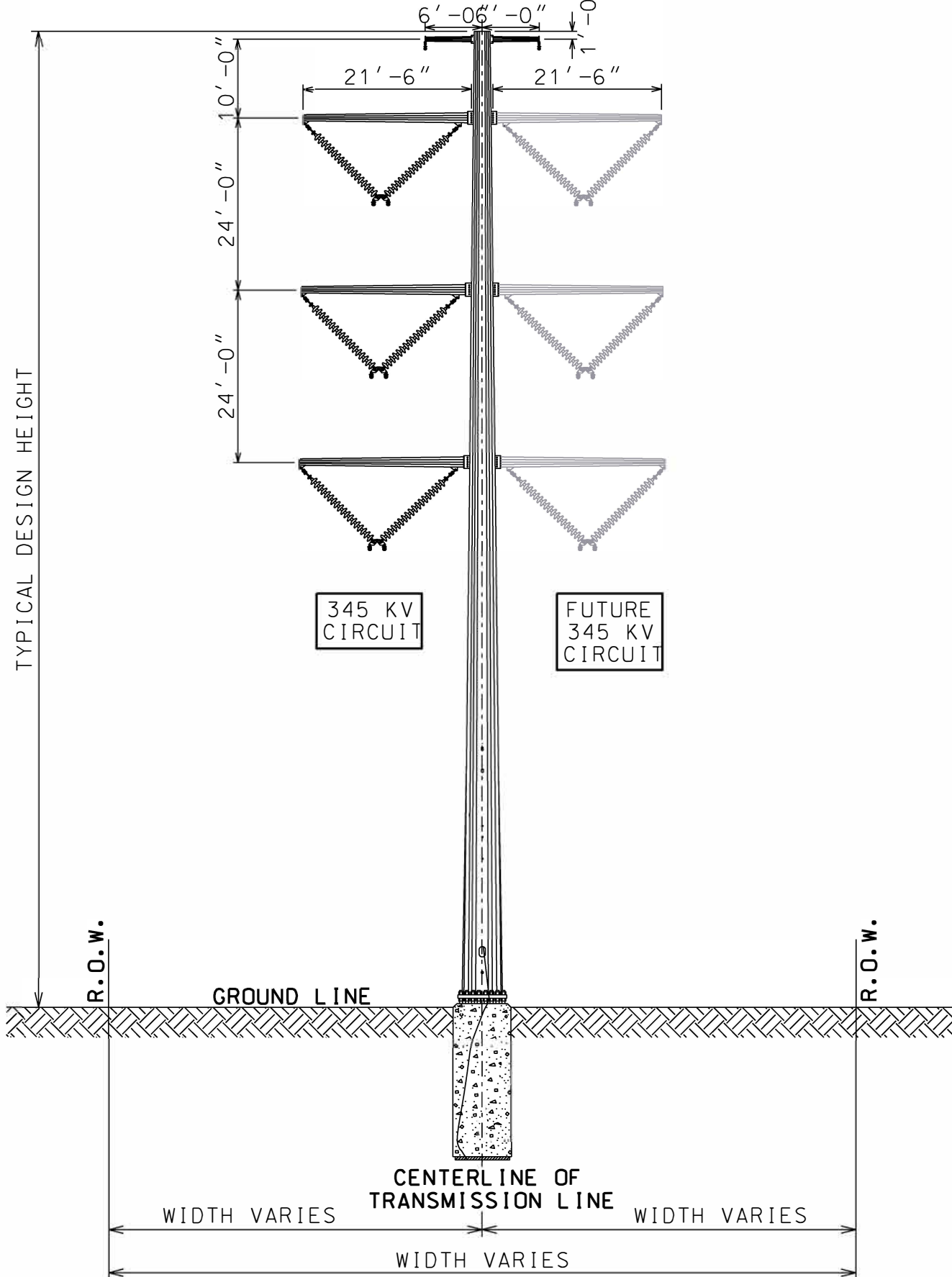
TYPICAL 345KV DOUBLE CIRCUIT TANGENT MONOPOLE NOT TO SCALE
