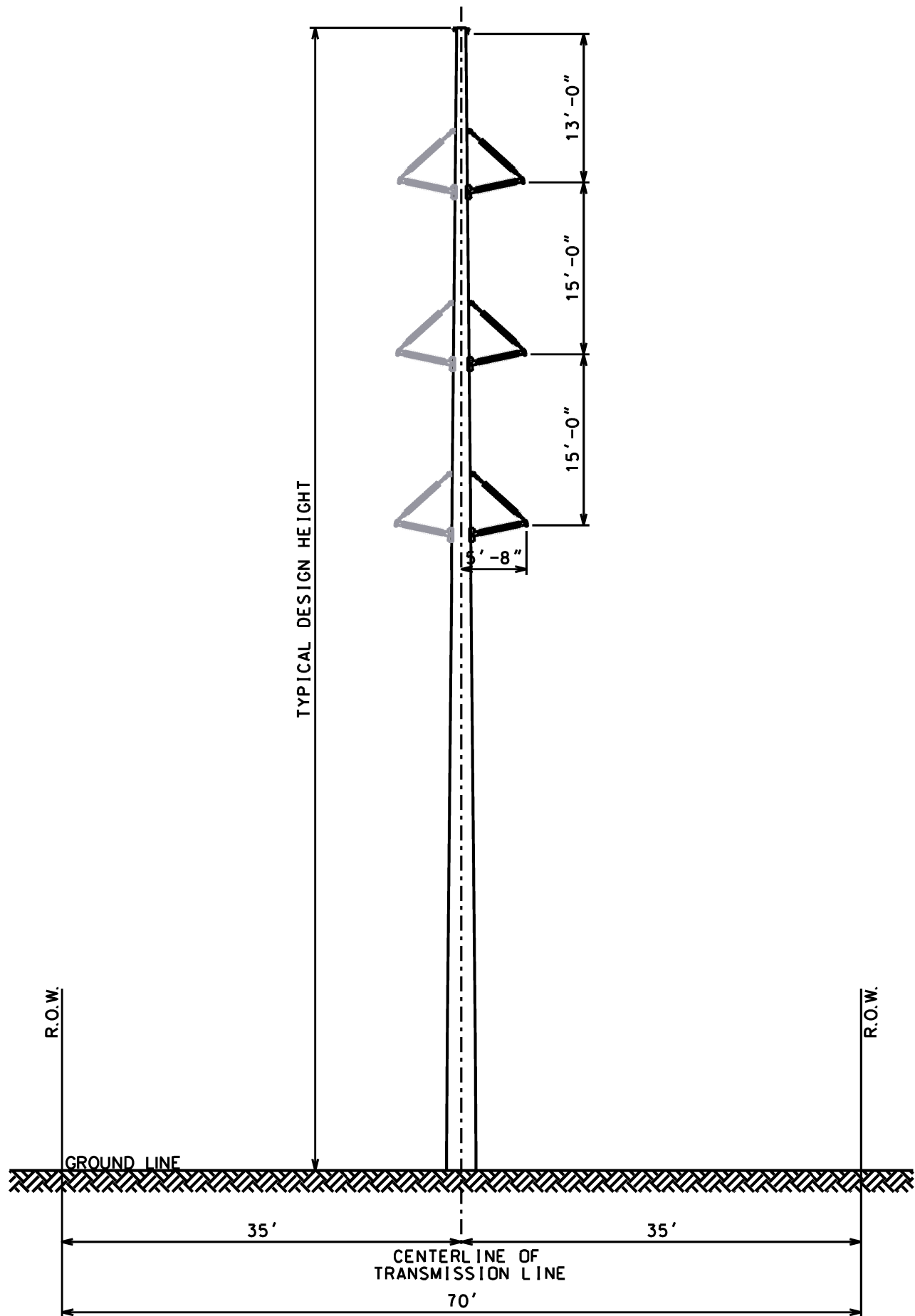
TYPICAL 138 KV TANGENT DOUBLE-CIRCUIT MONOPOLE WITH ONE CIRCUIT IN PLACE (NOT TO SCALE)
