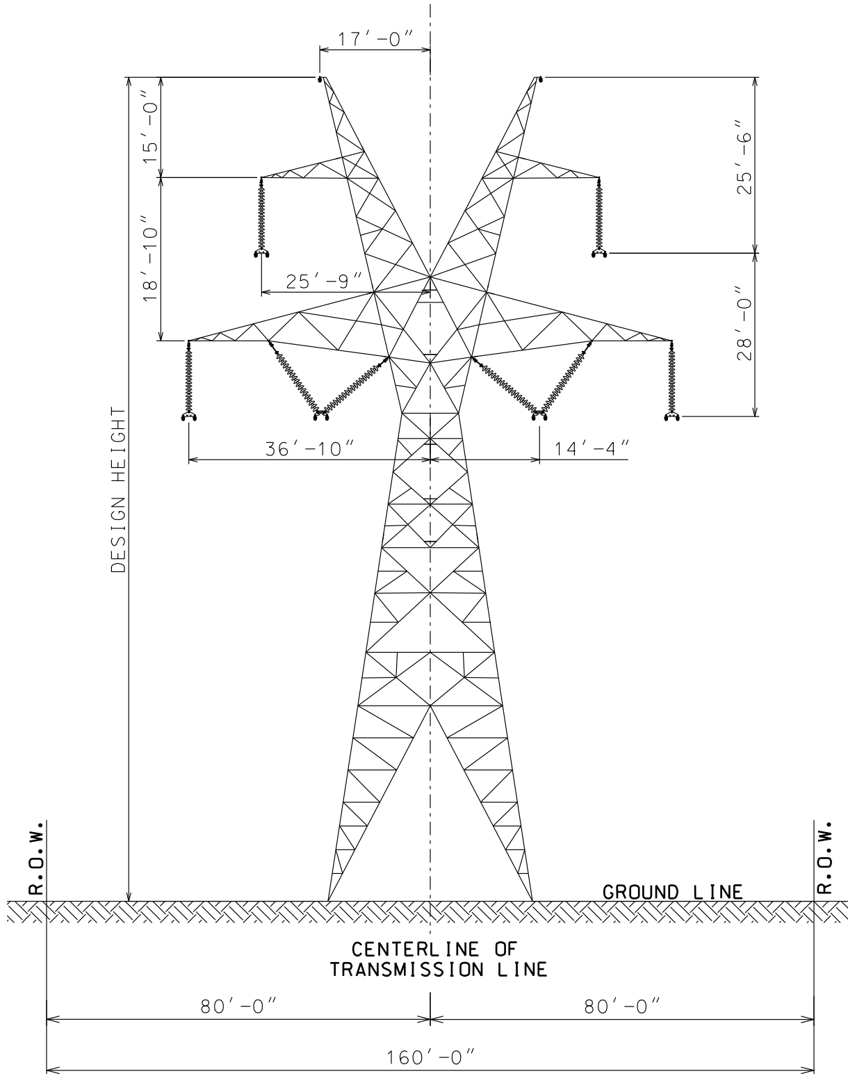
TYPICAL 345KV DOUBLE CIRCUIT TANGENT TOWER
