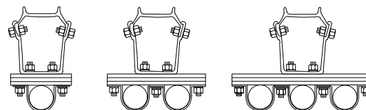
Typical Single Riser Installation
